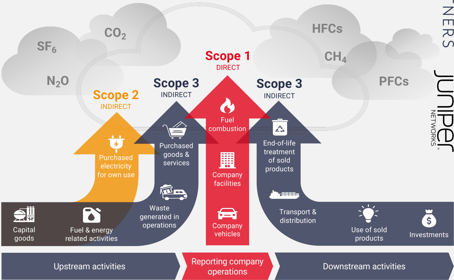
Figure 1: Classification of greenhouse gas emissions
