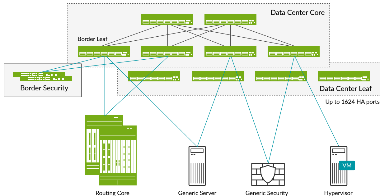
Figure 1: Building blocks help create repeatable, scalable data center designs by combining Juniper data center switches with Apstra fabric management software.
