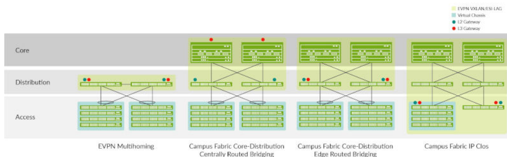
Figure 2: QFX10000 as distribution and core in EVPN multihoming and campus fabric architectures
