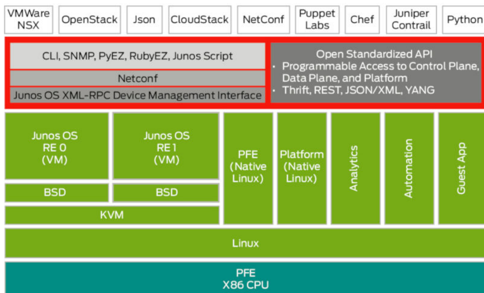
Figure 4: Juniper Programmability Framework
